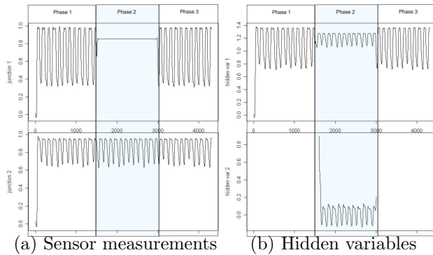
Figure 1: Illustration of problem. Sensors measure chlorine in drinking water and show a daily, near sinusoidal periodicity during phases 1 and 3. During phase 2, some of the sensors are “stuck” due to a major leak. The extra hidden variable introduced during phase 2 captures the presence of a new trend. SPIRIT can also tell us which sensors participate in the new, “abnormal” trend (e.g., close to a construction site). In phase 3, everything returns to normal.
